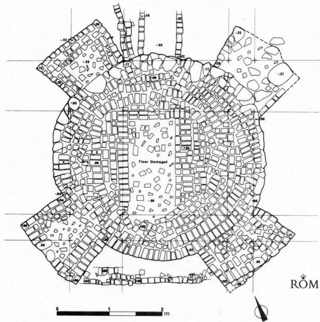
EGMONDVILLE POTTERY KILN
